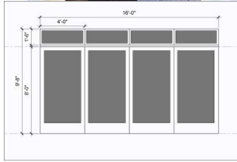
Sliding Doors in 4'x10' panels with transom & black frames in Great Room
